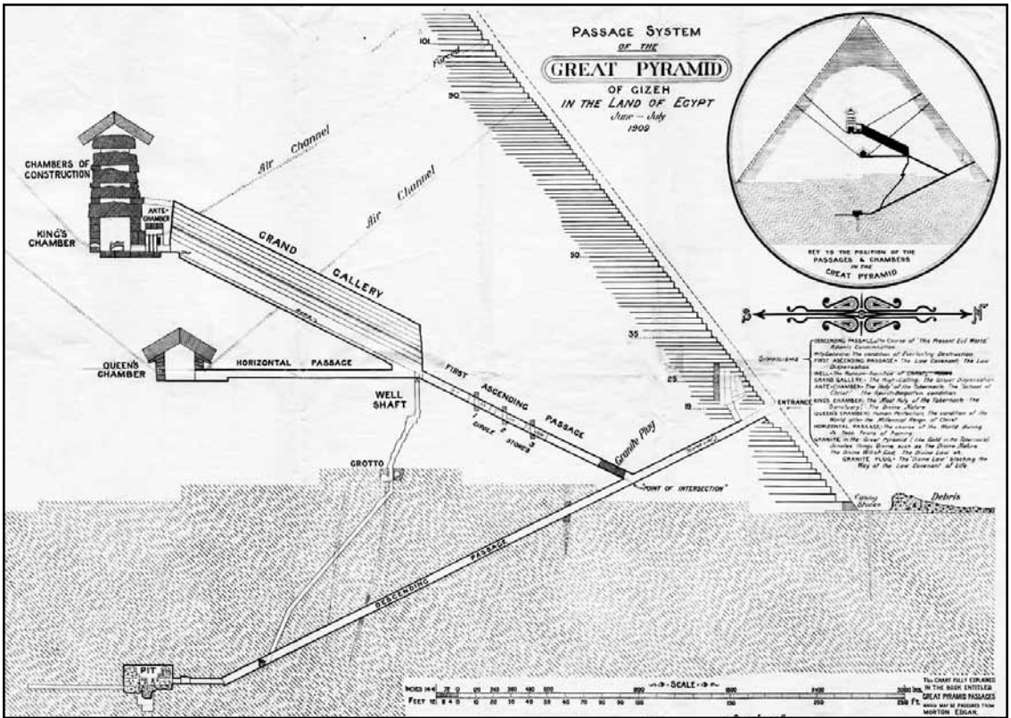
Figure 10.15 – The Edgar brother’s 1909 chart showing the Passages and Chambers.
