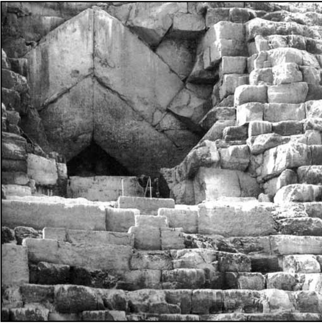
Figure 10.18 – The original entrance to the Descending Passage was originally concealed by a hinged casing stone.
