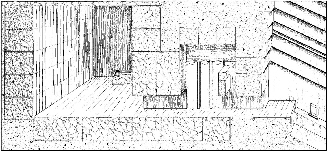
Figure 10.21 – Cut away, close-up view of the King's Chamber and Ante-Chamber showing the Granite Leaf and the use of red granite throughout. The Great Step and the southern portion of the Grand Gallery are also shown. Illustration 1933 by Howard B. Rand, used with permission.
