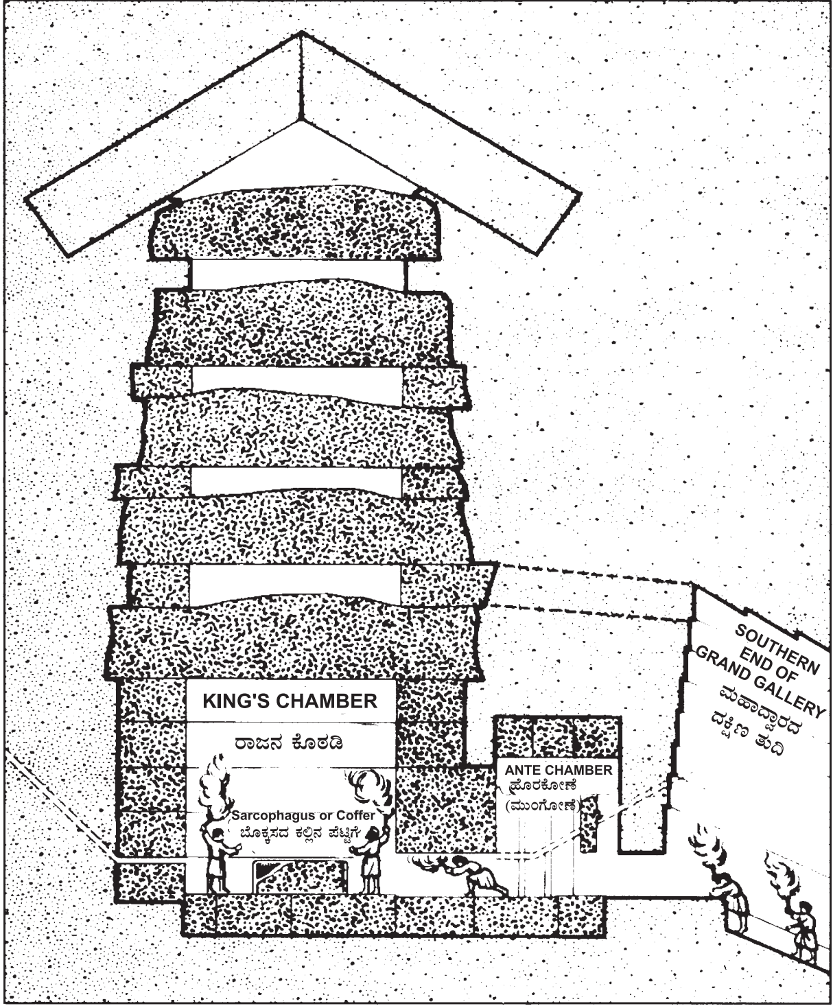
Vertical Section (looking west) of KING'S CHAMBER; also of ANTE-CHAMBER, South End of GRAND GALLERY and Vyse's Hollows of Construction above King's Chamber THE DARK TONED AREAS INDICATE GRANITE
